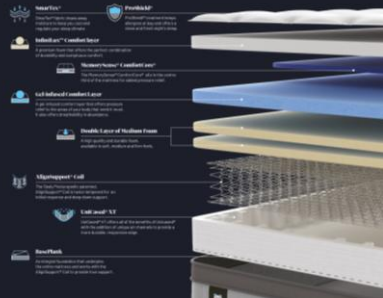
Image 5 Layer Diagram
